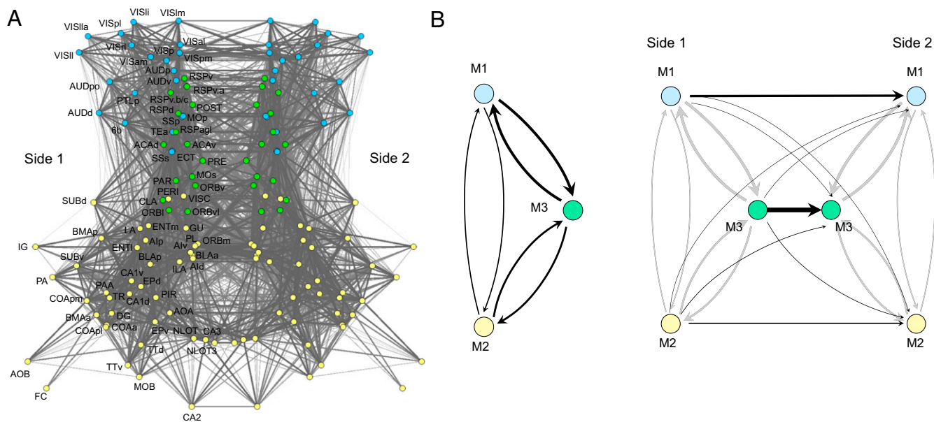
Fig. 5. Connection pattern layout diagrams. (A) The complete bilateral network of association and commissural connections. Nodes (regions) are projected onto two dimensions, using a Fruchterman–Reingold energy minimization layout algorithm. Nodes are color-coded by module assignment (M1, blue; M2, yellow; M3, green). To simplify the plot, connections are drawn without reference to directionality (gray level and thickness of line proportional to \log_{10} of connection weight). (B) Summary layout of aggregated connection weights between modules M1–M3 in one hemisphere (Left) and from modules M1–M3 on side 1 to modules M1–M3 on side 2 (Right). Arrows show directionality of connections, and their thickness is proportional to the average connection weights of between-module connections (Tables S1 and S3). Abbreviations are defined in Datasets S1 and S3 (worksheet 2).
