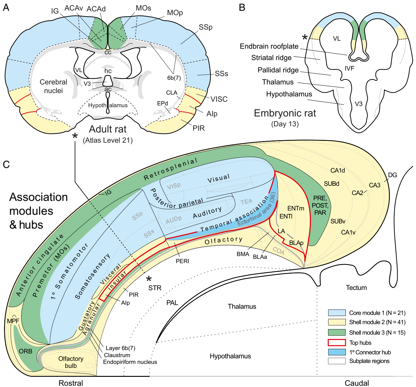
Fig. 6. Mapping the spatial distribution of modules and hubs in the rat. A shows the general localization of cortical regions and the cortical plate parts of M1–M3 (color coded) on a transverse section from the standard brain atlas used to create connection reports for this analysis. B is a fate map of presumed module localization on a transverse section of the forebrain vesicle on embryonic day 13. C shows the spatial extent of M1–3, the top-ranked hubs, including the primary connector hub, on a regionalized flat map of the right cerebral cortex. Note the basic core and shell arrangement of modules, with M1 (blue) forming a lateral core, and M2 (yellow) and M3 (green) forming (respectively) ventral and dorsal segments of the shell. The cortical subplate forms a deep layer 6b (or 7) of the cerebral cortex and as such is nested (gray outline) in the overall cortical plate representation (28). The topographic distributions in A and B serve primarily to help understand the flat-map topology (see the asterisk and dashed line in C , and the corresponding asterisks in A and B ). For high-resolution details of the flat map, see ref. 28. Abbreviations are defined in Datasets S1 and S3 (worksheet 2). A and C are adapted from ref. 28, and B is adapted from ref. 29.
